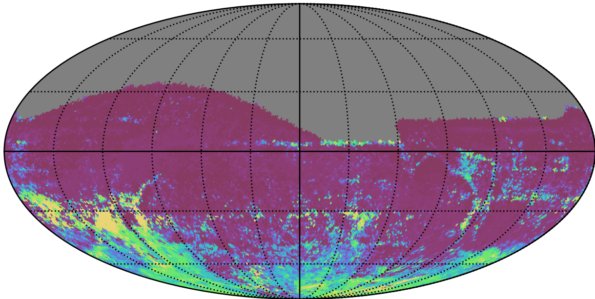
no_high_blob_v3.3_10yrs All sky r band: 75th Percentile Intranight Timespan
