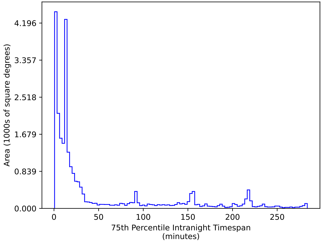
no_high_blob_v3.3_10yrs All sky r band: 75th Percentile Intranight Timespan
