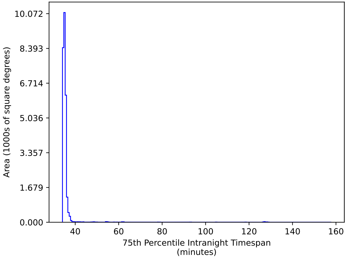
no_high_blob_v3.3_10yrs All sky iz bands: 75th Percentile Intranight Timespan
