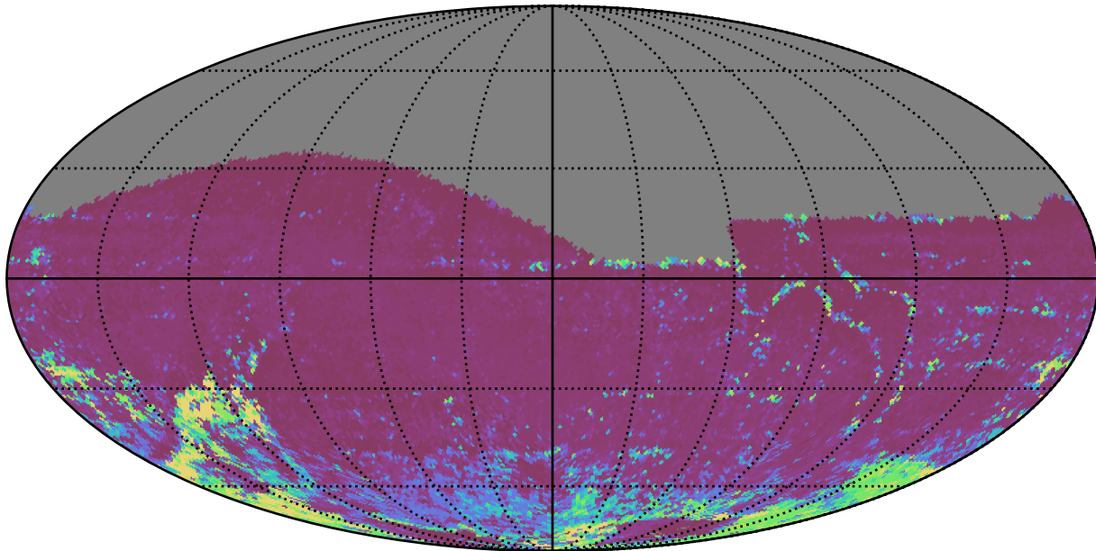
no_high_blob_v3.3_10yrs All sky i band: 75th Percentile Intranight Timespan
