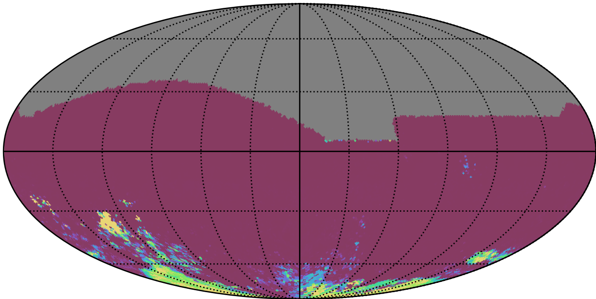
no_high_blob_v3.3_10yrs All sky gr bands: 75th Percentile Intranight Timespan
