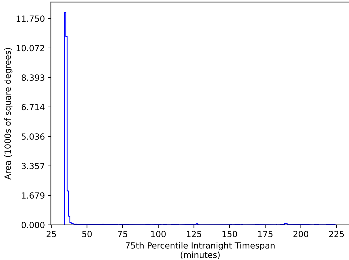
no_high_blob_v3.3_10yrs All sky gr bands: 75th Percentile Intranight Timespan
