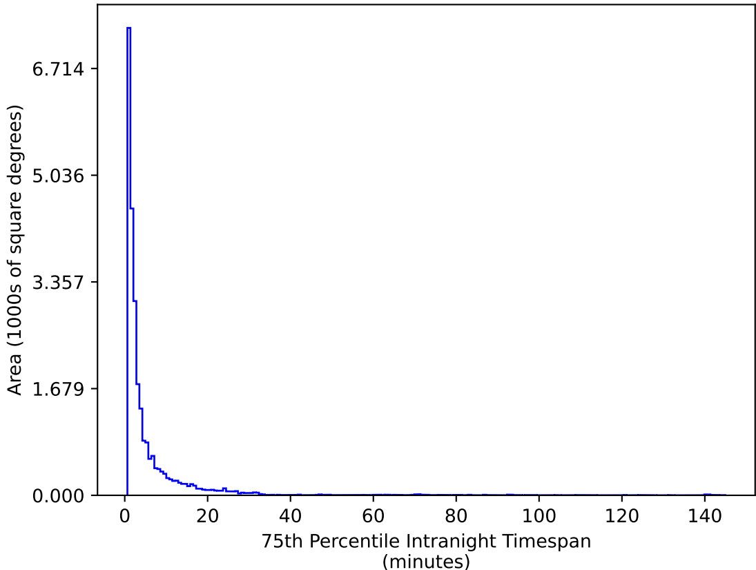
no_high_blob_v3.3_10yrs All sky g band: 75th Percentile Intranight Timespan
