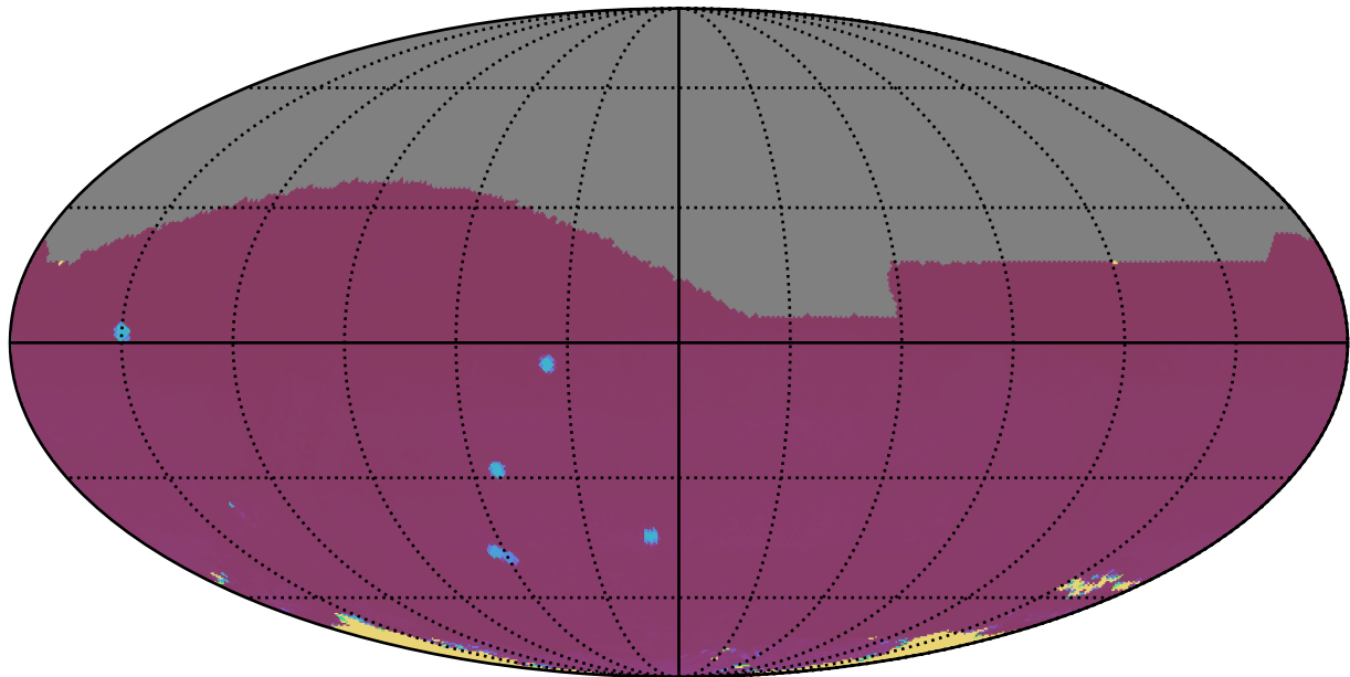
no_high_blob_v3.3_10yrs All sky all bands: 75th Percentile Intranight Timespan
