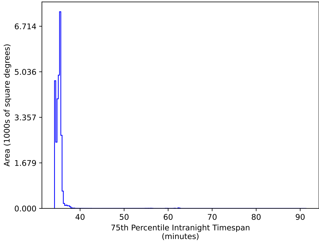
no_high_blob_v3.3_10yrs All sky all bands: 75th Percentile Intranight Timespan
