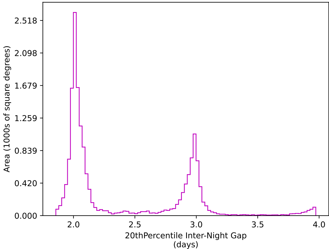
no_high_blob_v3.3_10yrs WFD z band: 20thPercentile Inter-Night Gap
