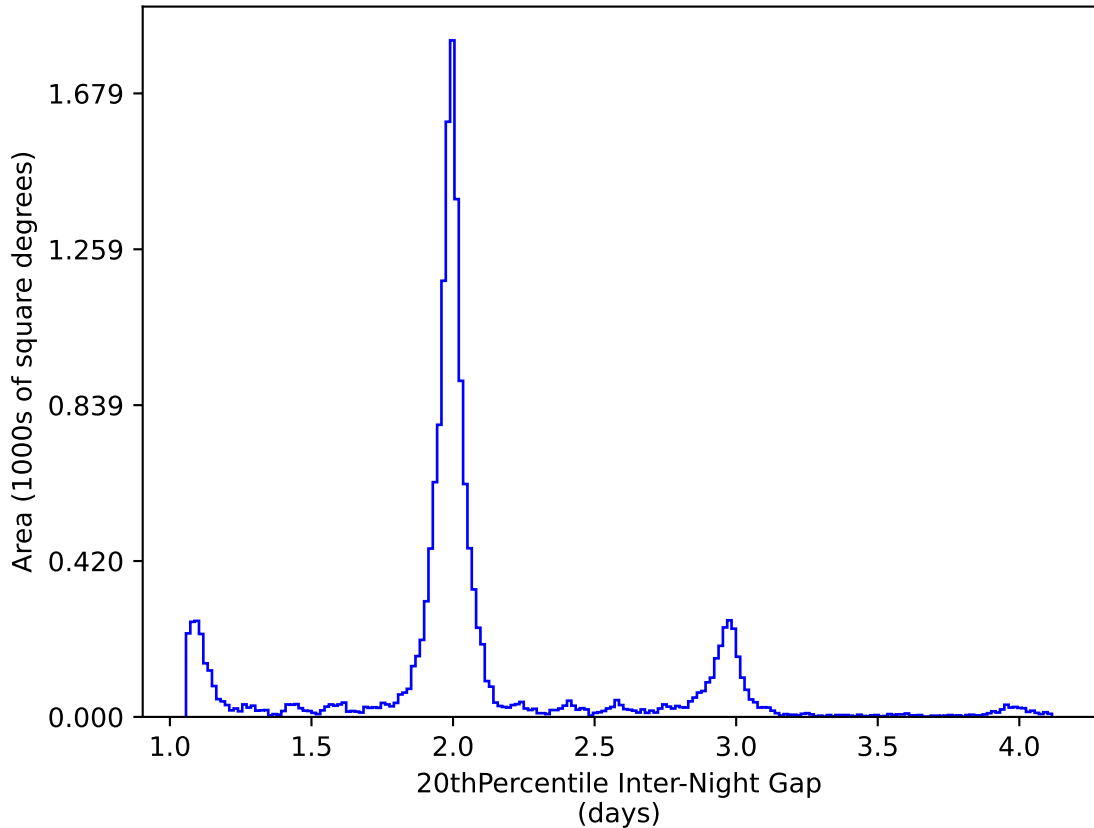
no_high_blob_v3.3_10yrs WFD y band: 20thPercentile Inter-Night Gap
