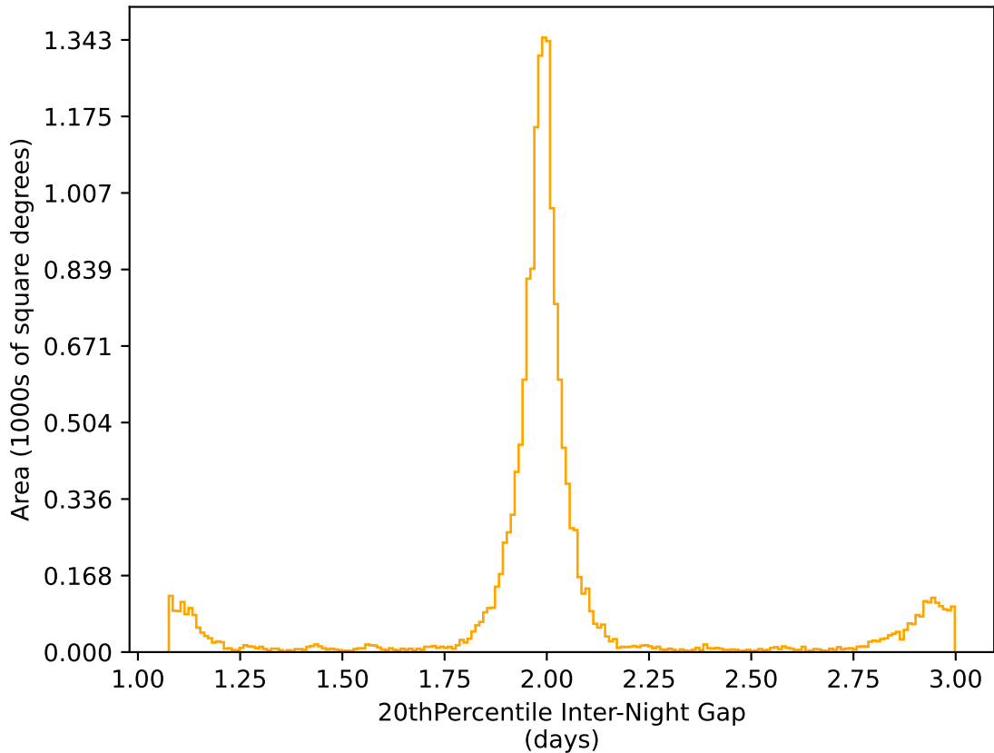
no_high_blob_v3.3_10yrs WFD r band: 20thPercentile Inter-Night Gap
