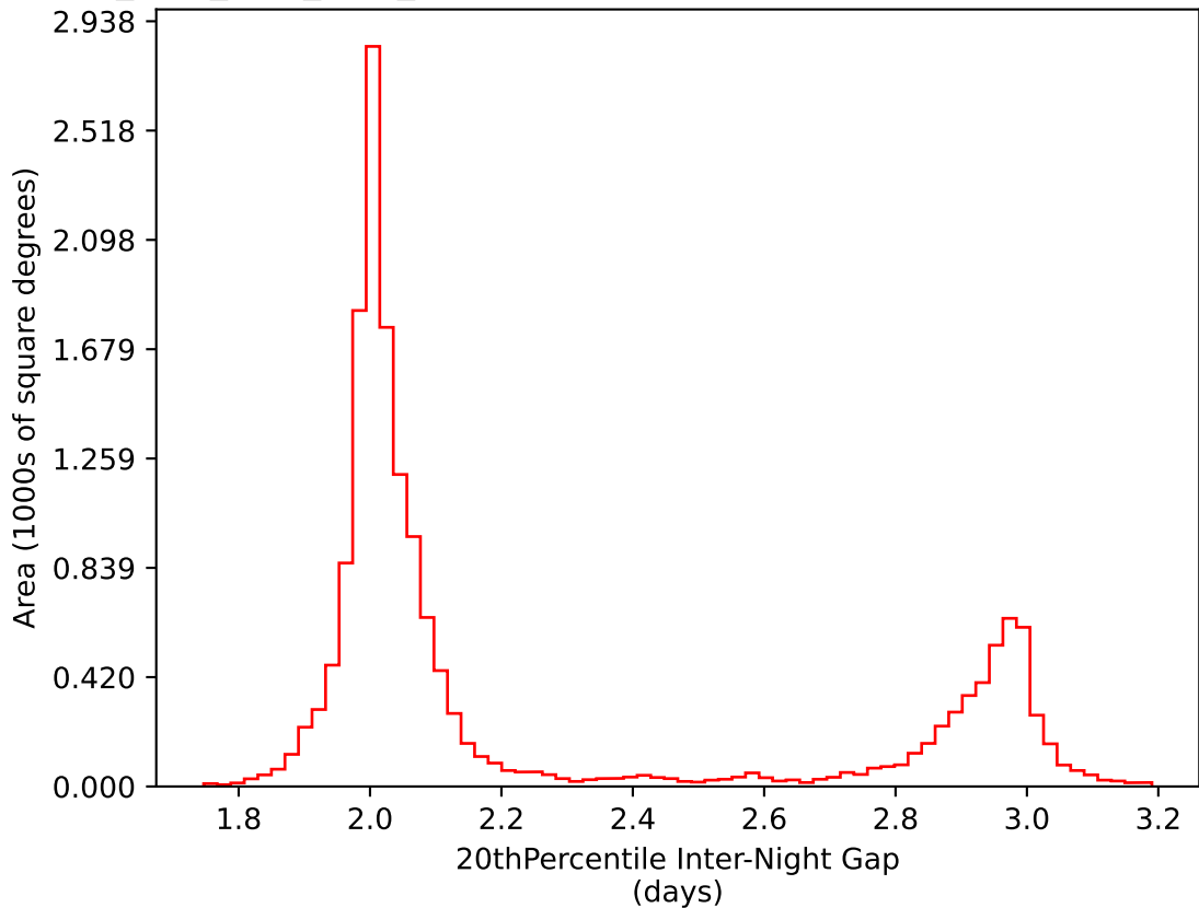
no_high_blob_v3.3_10yrs WFD i band: 20thPercentile Inter-Night Gap
