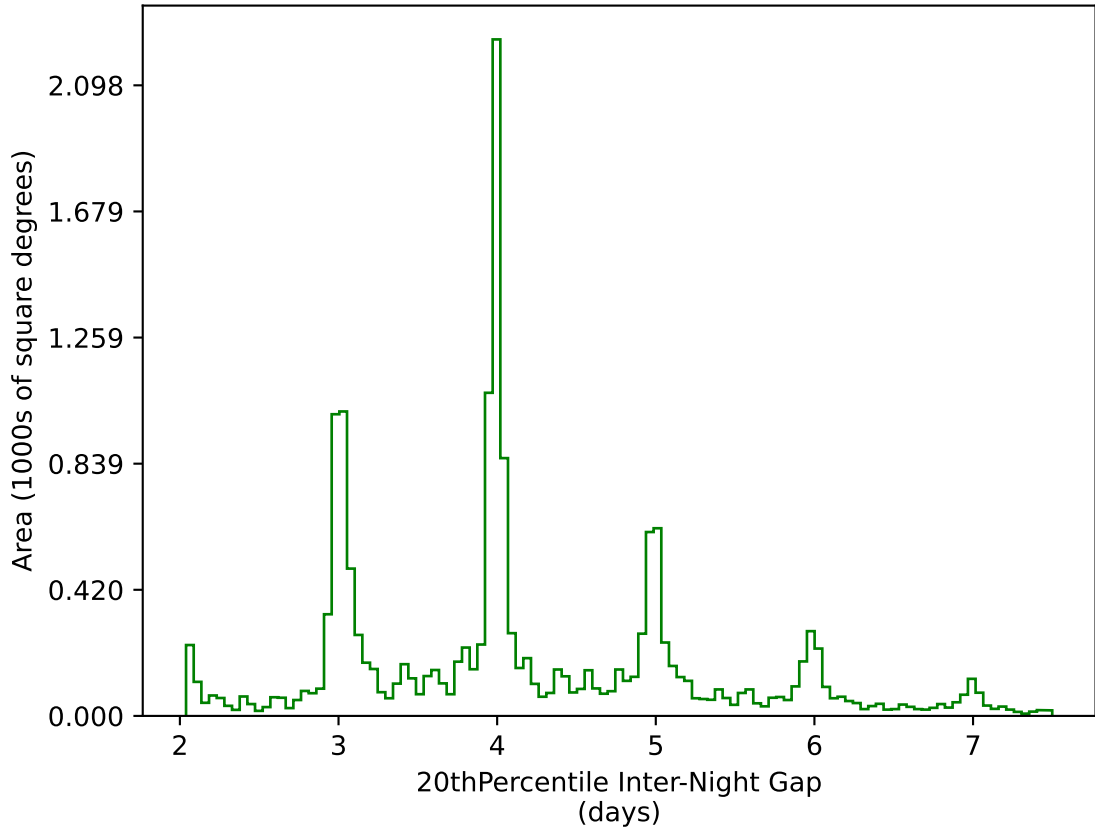
no_high_blob_v3.3_10yrs WFD g band: 20thPercentile Inter-Night Gap
