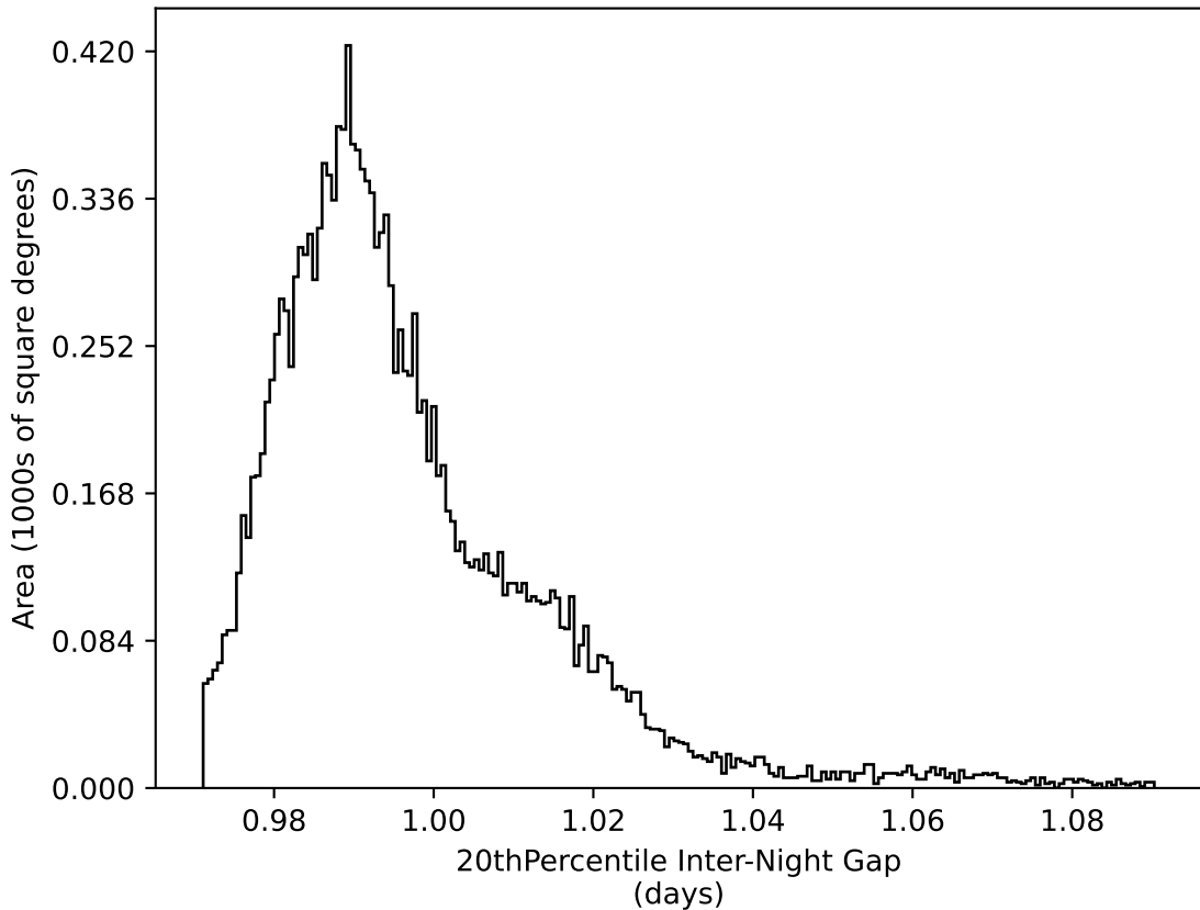
no_high_blob_v3.3_10yrs WFD all bands: 20thPercentile Inter-Night Gap
