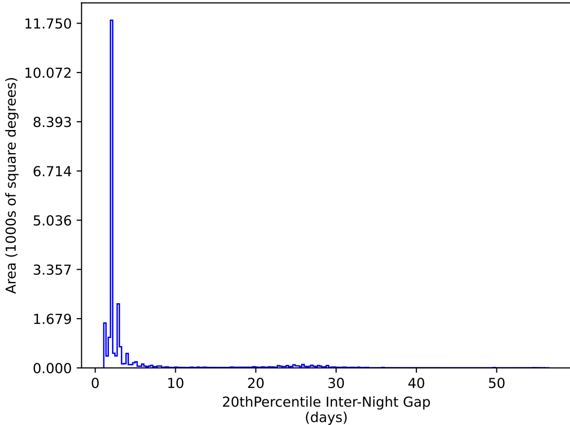
no_high_blob_v3.3_10yrs All sky y band: 20thPercentile Inter-Night Gap
