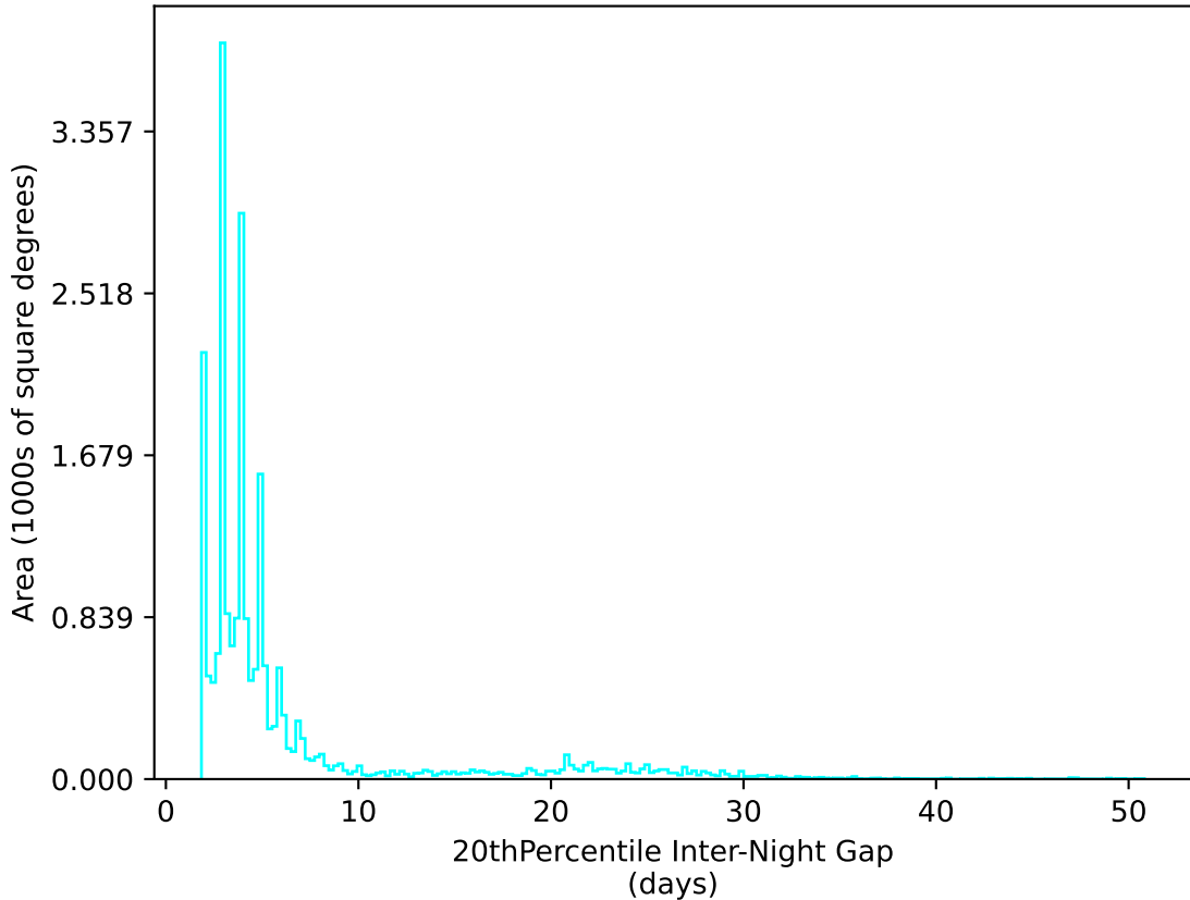
no_high_blob_v3.3_10yrs All sky u band: 20thPercentile Inter-Night Gap
