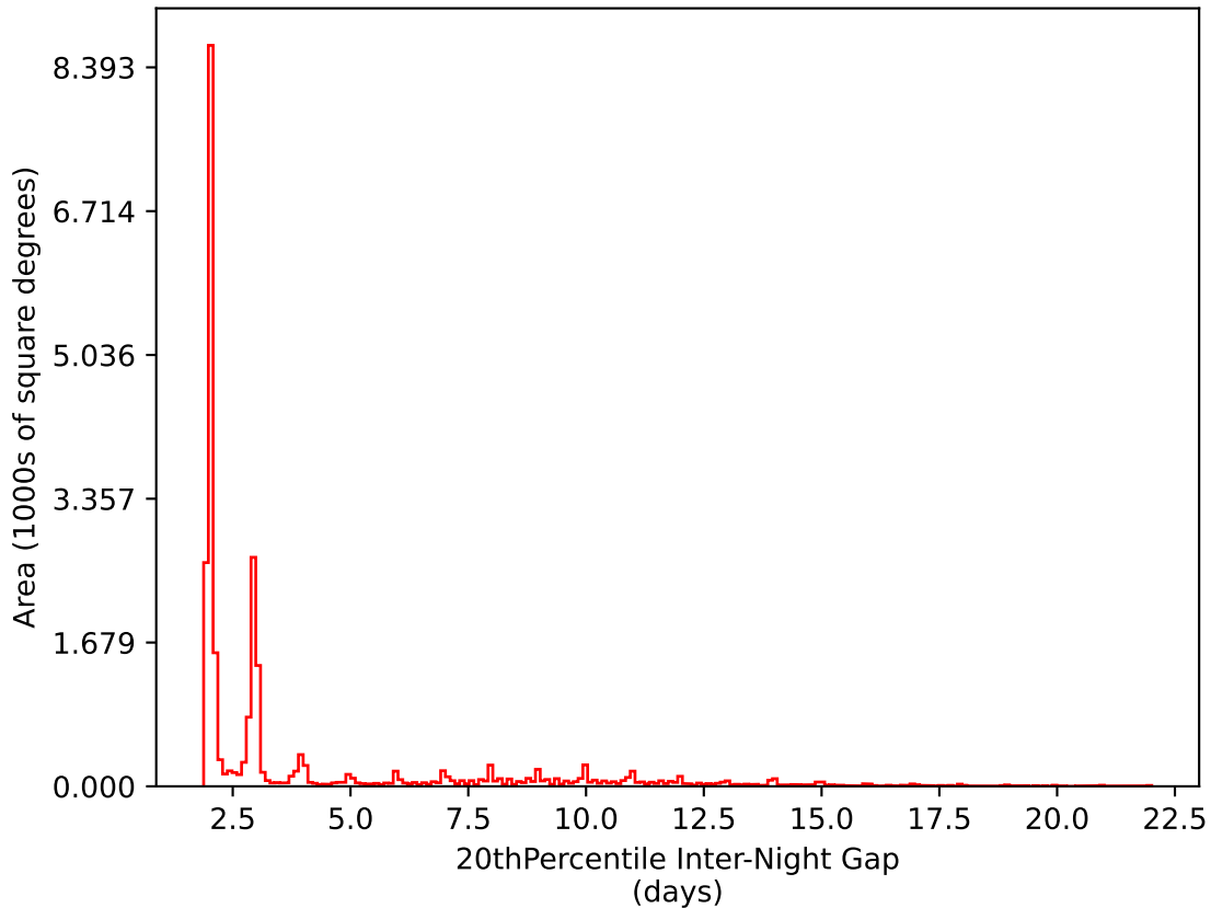
no_high_blob_v3.3_10yrs All sky i band: 20thPercentile Inter-Night Gap
