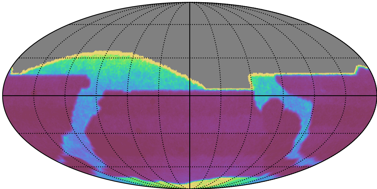
no_high_blob_v3.3_10yrs : properMotion
