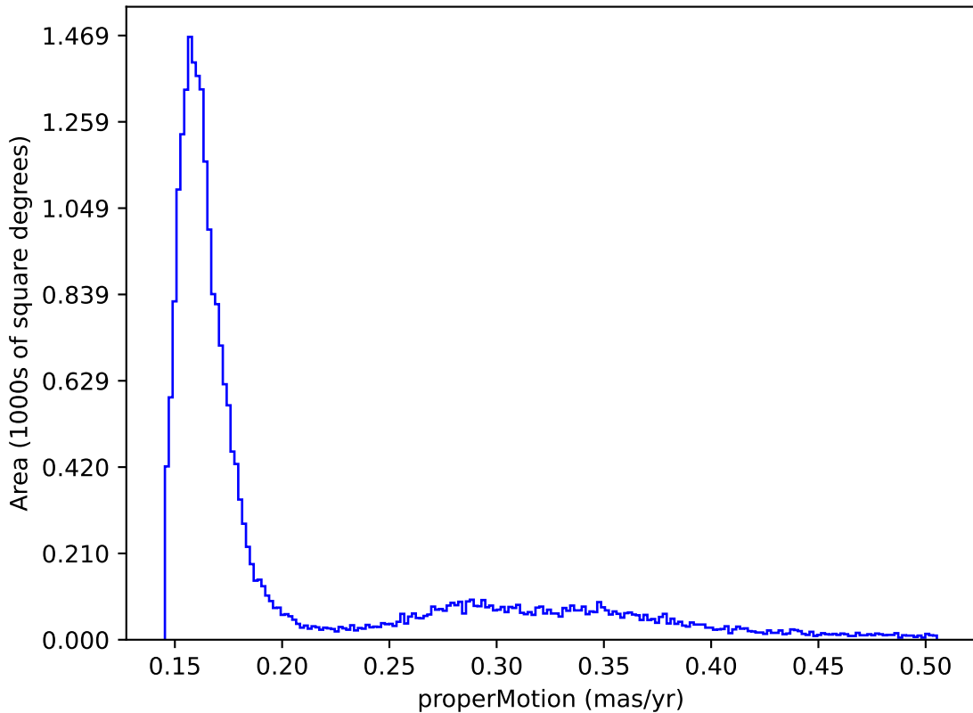
no_high_blob_v3.3_10yrs : properMotion
