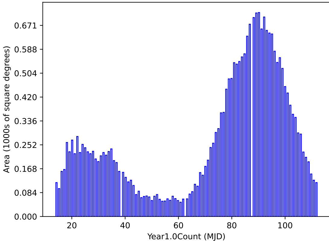
no_high_blob_v3.3_10yrs night &lt; 365.25: Year1.0Count
