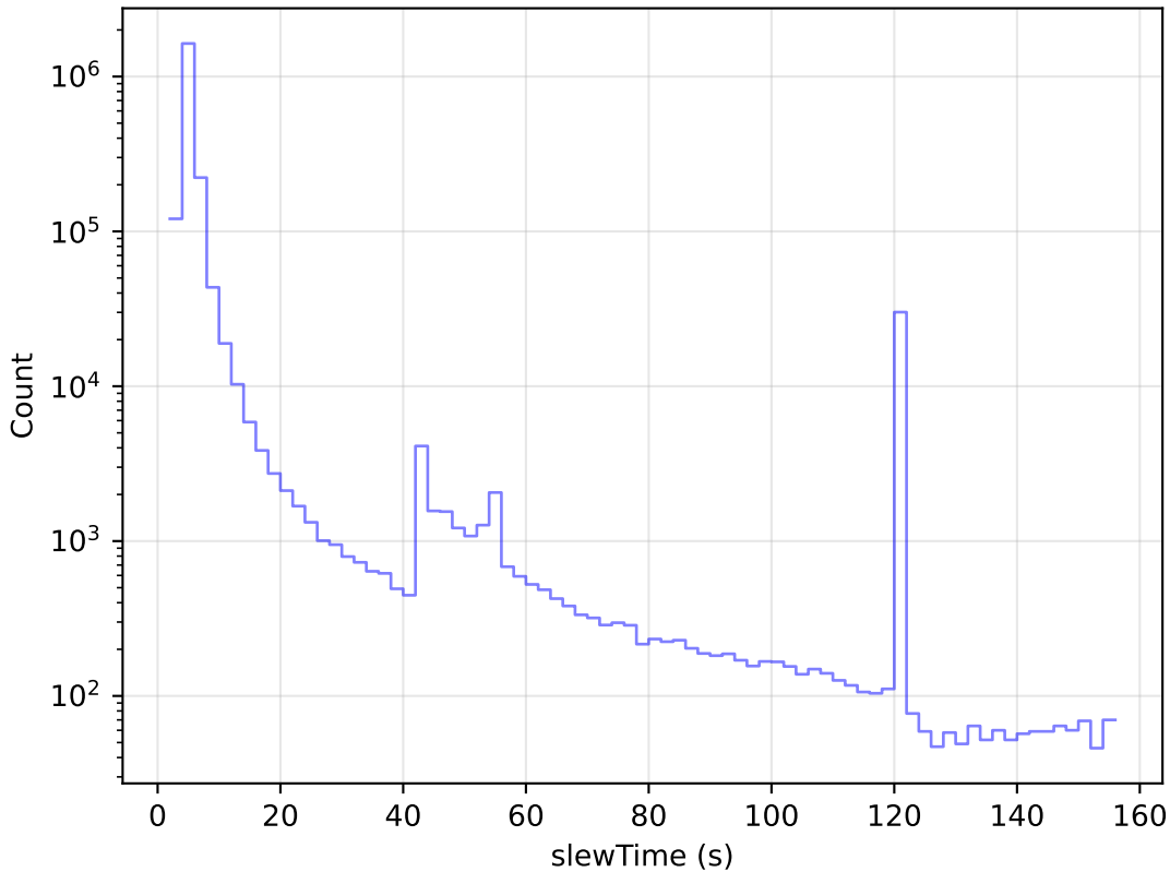
no_high_blob_v3.3_10yrs All visits: Slew Time Histogram
