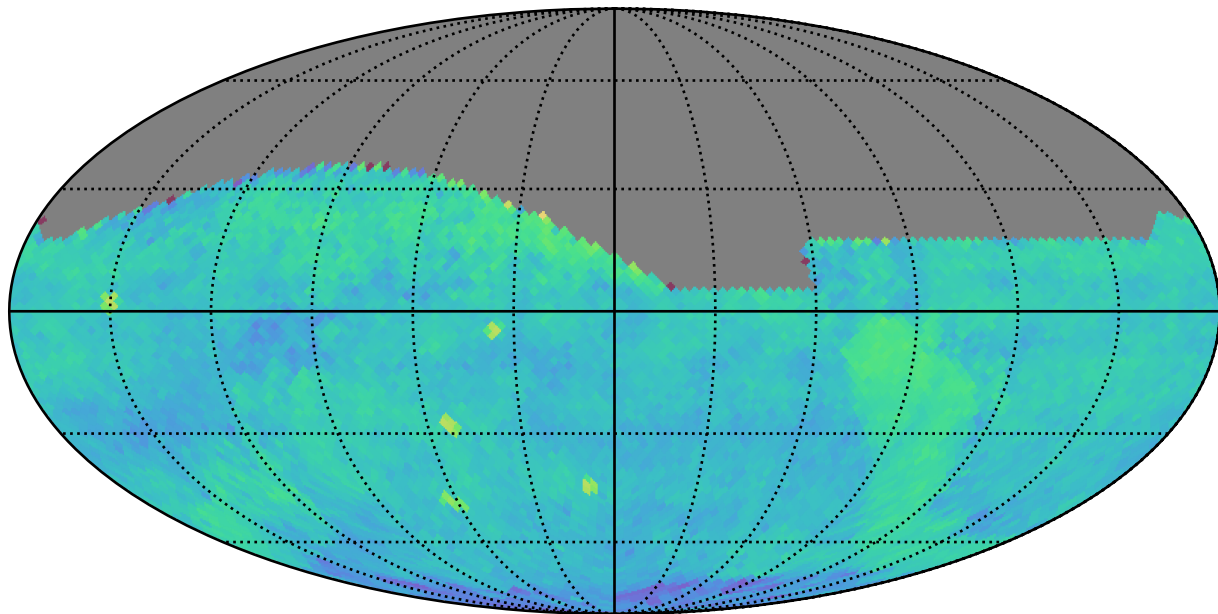
no_high_blob_v3.3_10yrs (g or r or i): PairFraction
