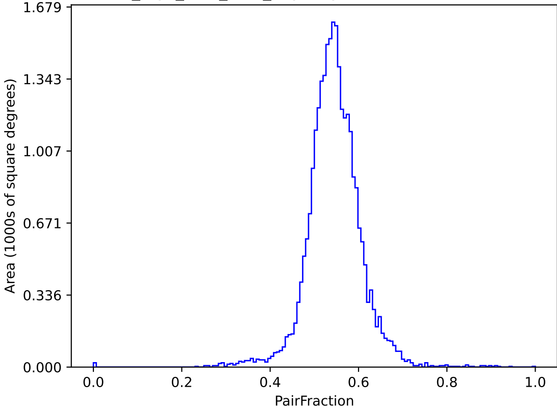
no_high_blob_v3.3_10yrs (g or r or i): PairFraction
