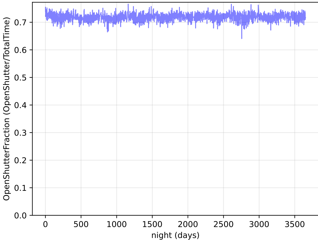
no_high_blob_v3.3_10yrs : OpenShutterFraction
