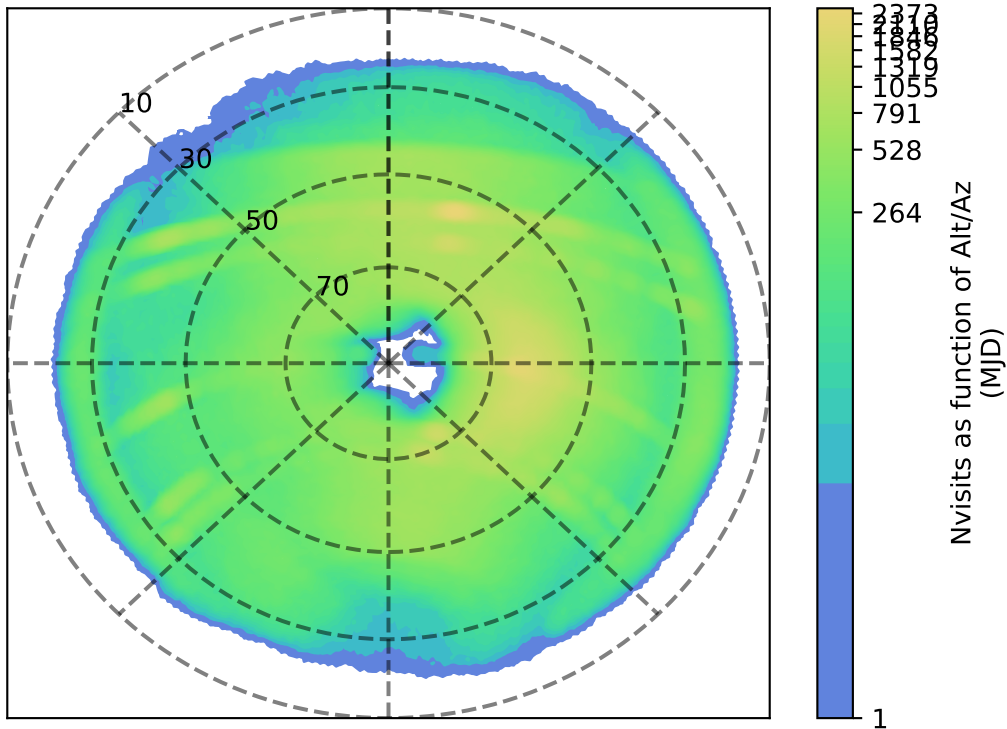
no_high_blob_v3.3_10yrs z: Nvisits as function of Alt/Az
