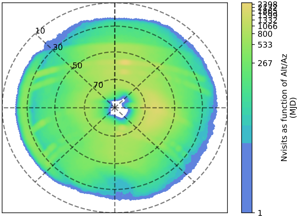
no_high_blob_v3.3_10yrs r: Nvisits as function of Alt/Az
