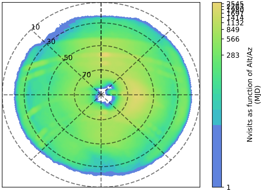
no_high_blob_v3.3_10yrs i: Nvisits as function of Alt/Az
