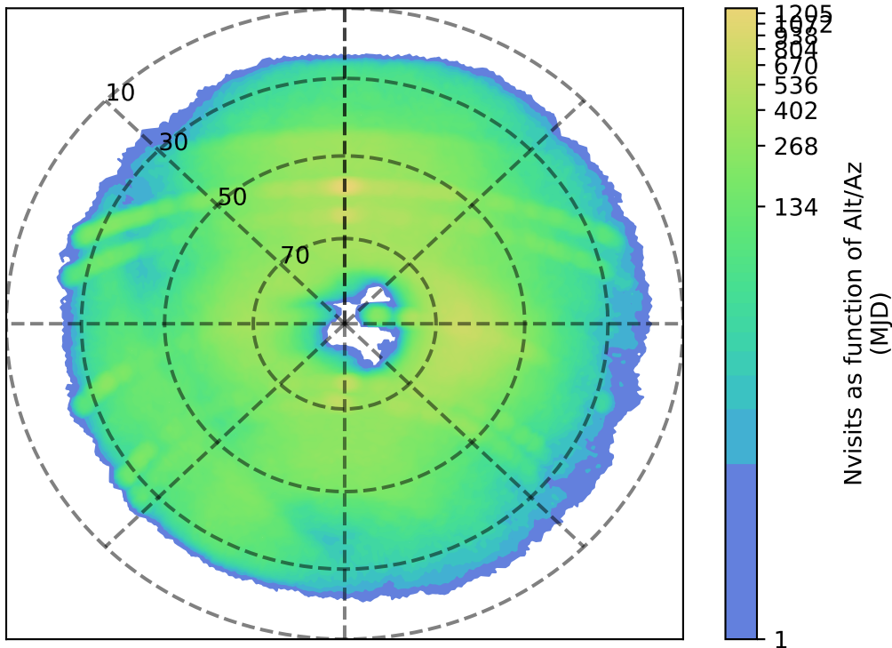
no_high_blob_v3.3_10yrs g: Nvisits as function of Alt/Az
