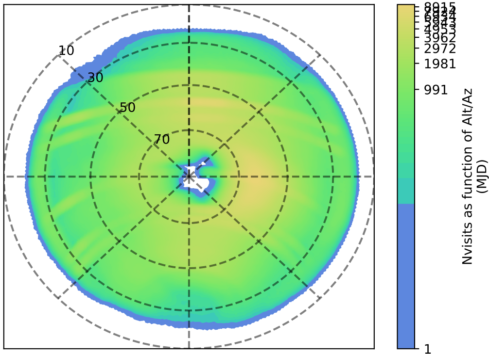
no_high_blob_v3.3_10yrs : Nvisits as function of Alt/Az
