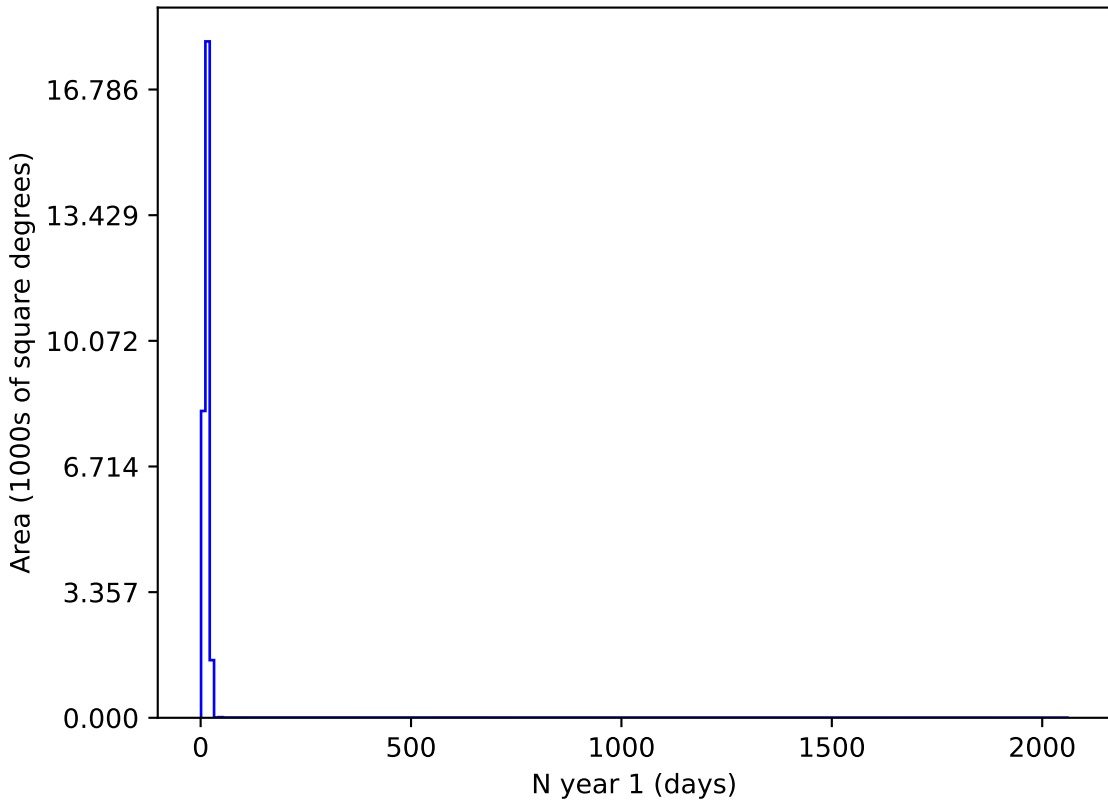
no_high_blob_v3.3_10yrs z and night < 365: N year 1
