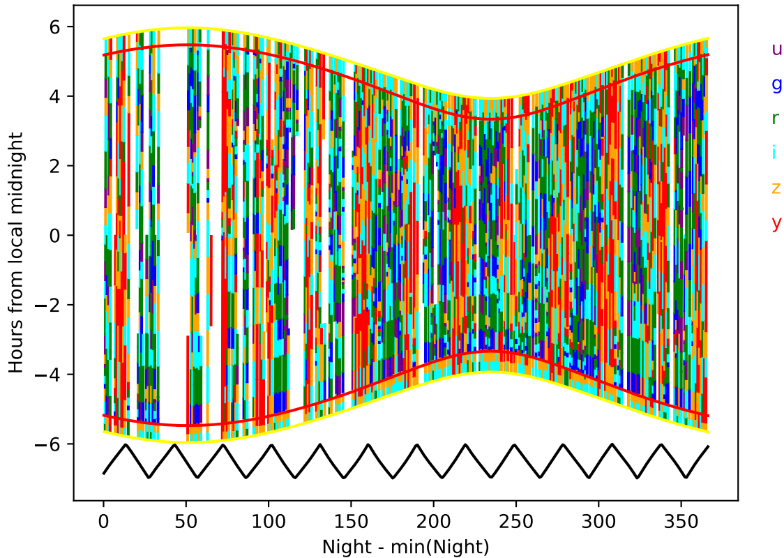
no_high_blob_v3.3_10yrs year 8-9: Hourglass
