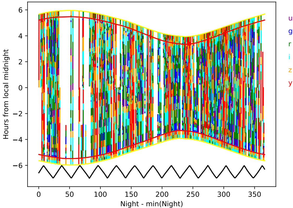
no_high_blob_v3.3_10yrs year 3-4: Hourglass
