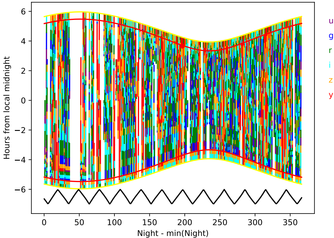
no_high_blob_v3.3_10yrs year 2-3: Hourglass
