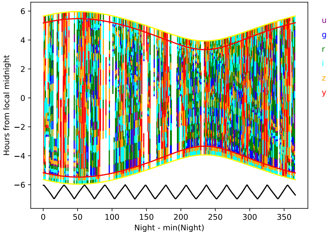
no_high_blob_v3.3_10yrs year 1-2: Hourglass
