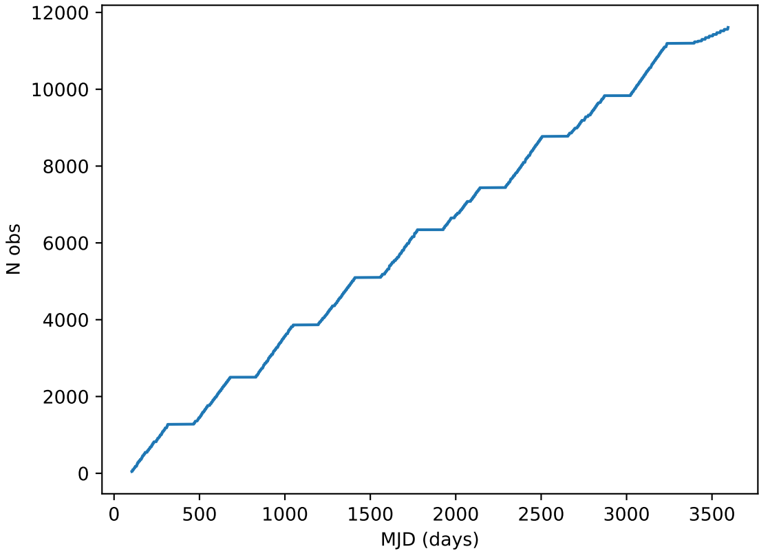
no_high_blob_v3.3_10yrs note like DD:EDFS_b%: Cumulative
