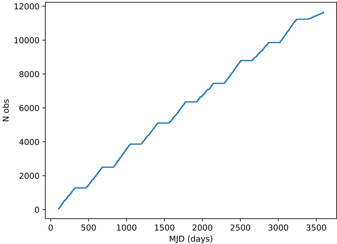
no_high_blob_v3.3_10yrs note like DD:EDFS_a%: Cumulative
