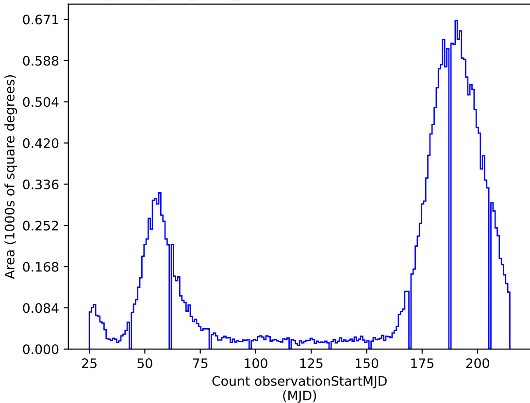
no_high_blob_v3.3_10yrs i: Count observationStartMJD
