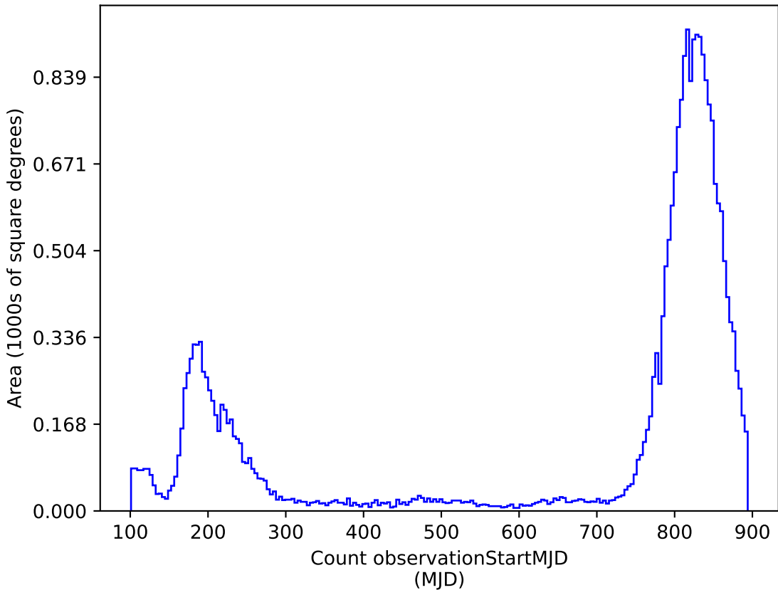
no_high_blob_v3.3_10yrs : Count observationStartMJD
