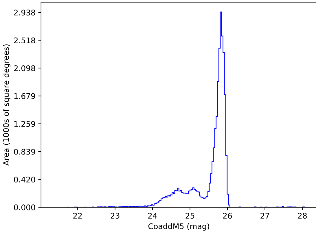
no_high_blob_v3.3_10yrs z: CoaddM5
