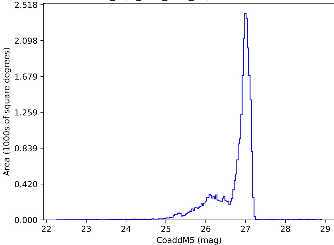
no_high_blob_v3.3_10yrs r: CoaddM5
