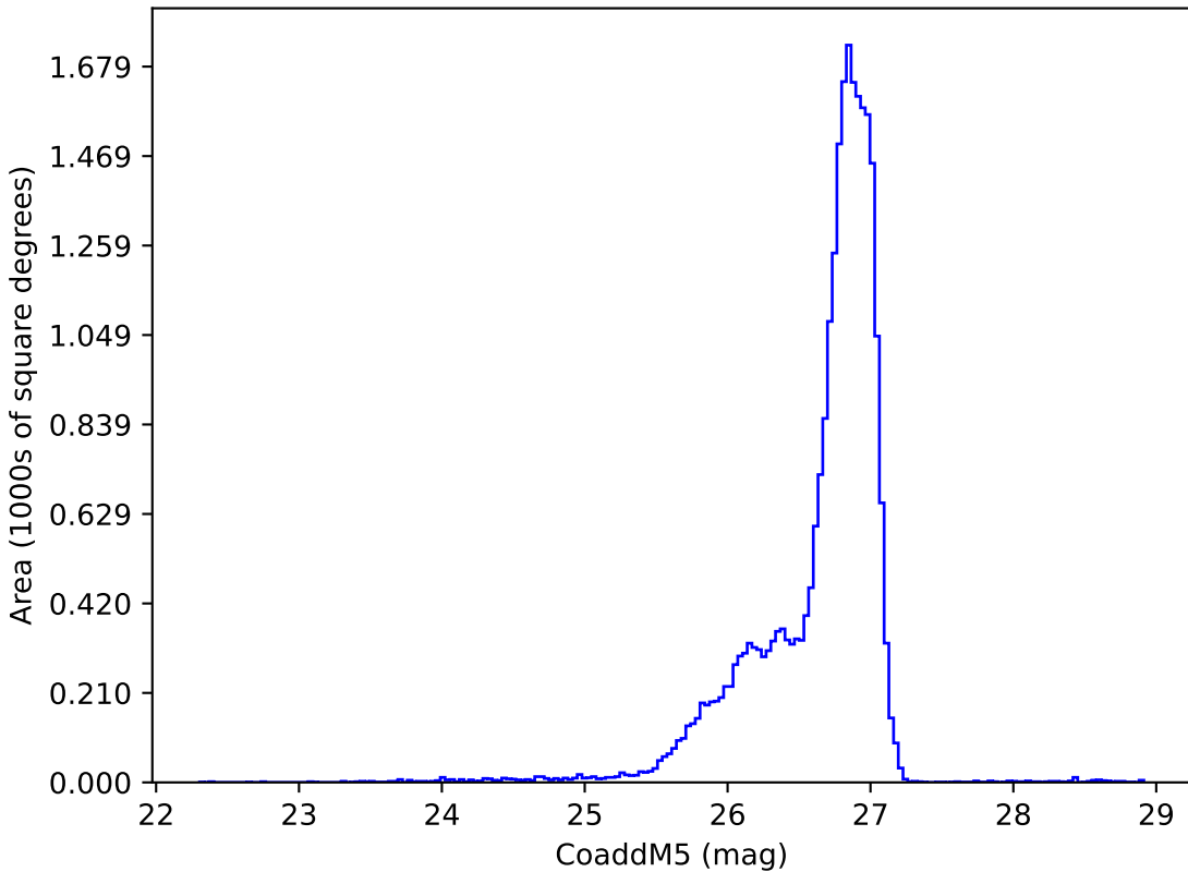
no_high_blob_v3.3_10yrs g: CoaddM5
