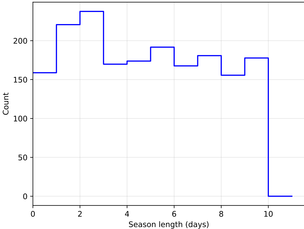
no_high_blob_v3.3_10yrs DD:WFD all bands: SeasonLength
