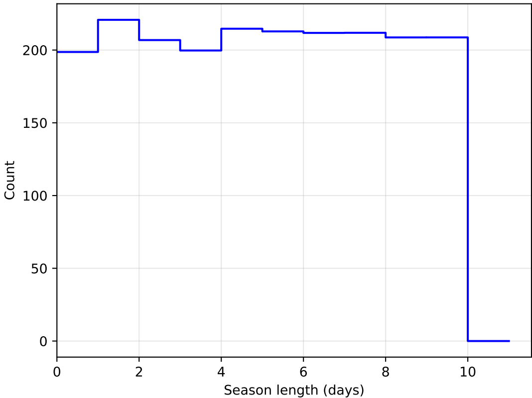
no_high_blob_v3.3_10yrs DD:ELAISS1 all bands: SeasonLength
