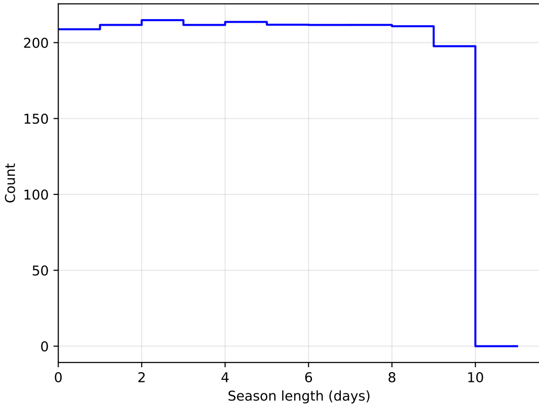
no_high_blob_v3.3_10yrs DD:EDFS all bands: SeasonLength
