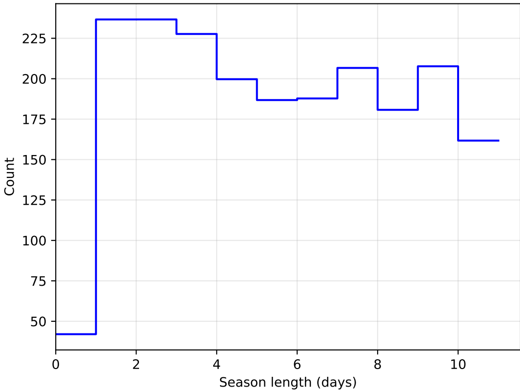
no_high_blob_v3.3_10yrs DD: COSMOS all bands: SeasonLength
