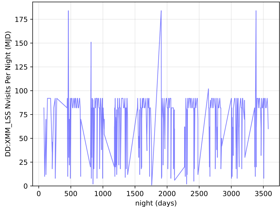
no_high_blob_v3.3_10yrs all bands: DD:XMM_LSS Nvisits Per Night
