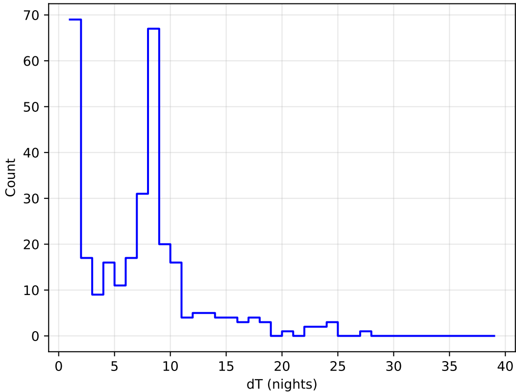
no_high_blob_v3.3_10yrs all bands: DD:XMM_LSS Delta Nights Histogram
