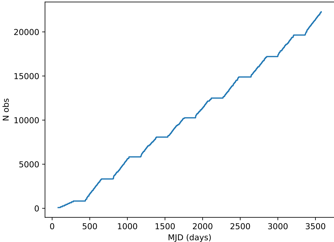
no_high_blob_v3.3_10yrs all bands: DD:XMM_LSS Cumulative NVisits
