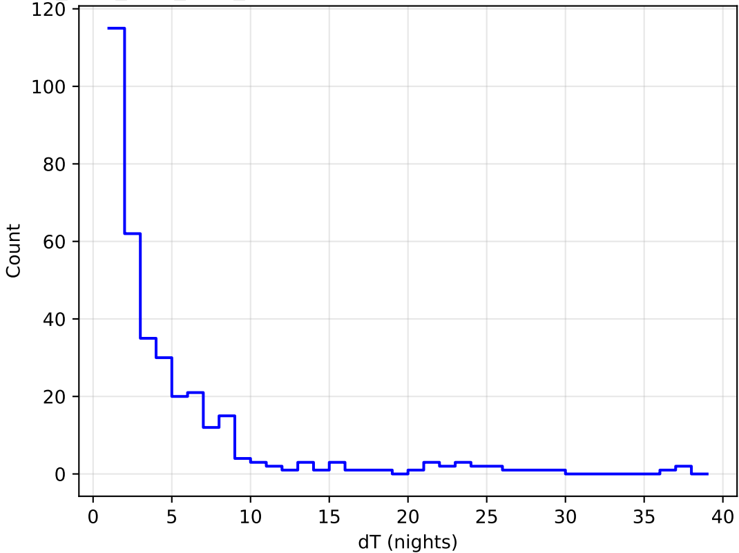
no_high_blob_v3.3_10yrs all bands: DD:WFD Delta Nights Histogram
